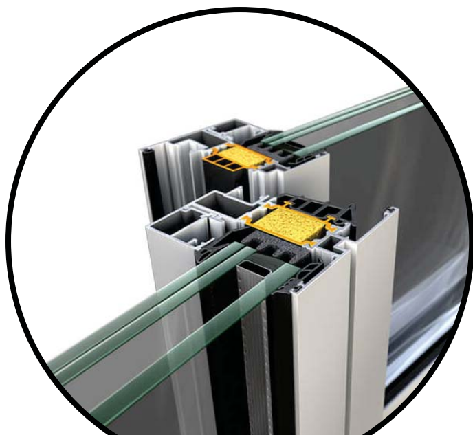
SUPREME S77 -alumil-
